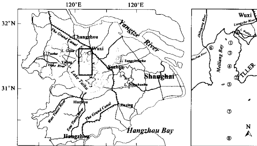
Fig.1 Map of Taihu Lake and its catchment showing the sampling sites 0—8. The point labeled “TLLER” marks the location of the Taihu Laboratory for Lake Ecosystem Research, in which all meteorological observation and analytical experiments were done in relation to this research
