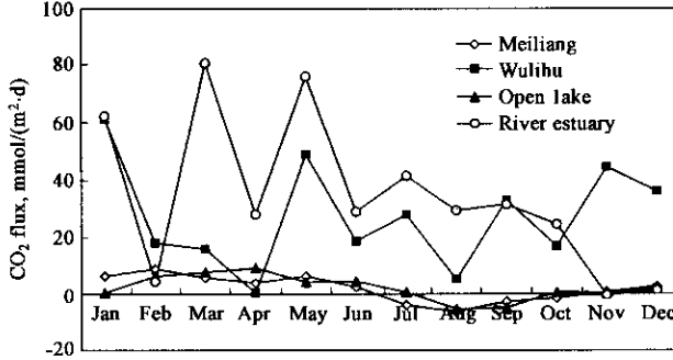
Fig.4 Monthly variation of atmospheric fluxes of \text{CO}_2 in different trophic lake areas in 1998
