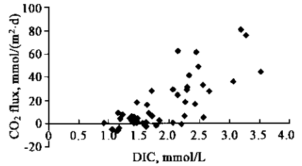
Fig.5 Distribution of atmospheric fluxes of \text{CO}_2 vs. dissolved inorganic carbon in the Taihu Lake in 1998
