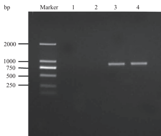
Fig. 1 Amplification of arsM by RT-PCR. Samples were detected for arsM gene, vector plasmid pET28a+ (lane 1) and arsM gene (lane 3) was overexpressed in B. idriensis ; vector plasmid pET28a+ (lane 2) and arsM gene (lane 4) was overexpressed in S. desiccabilis .
