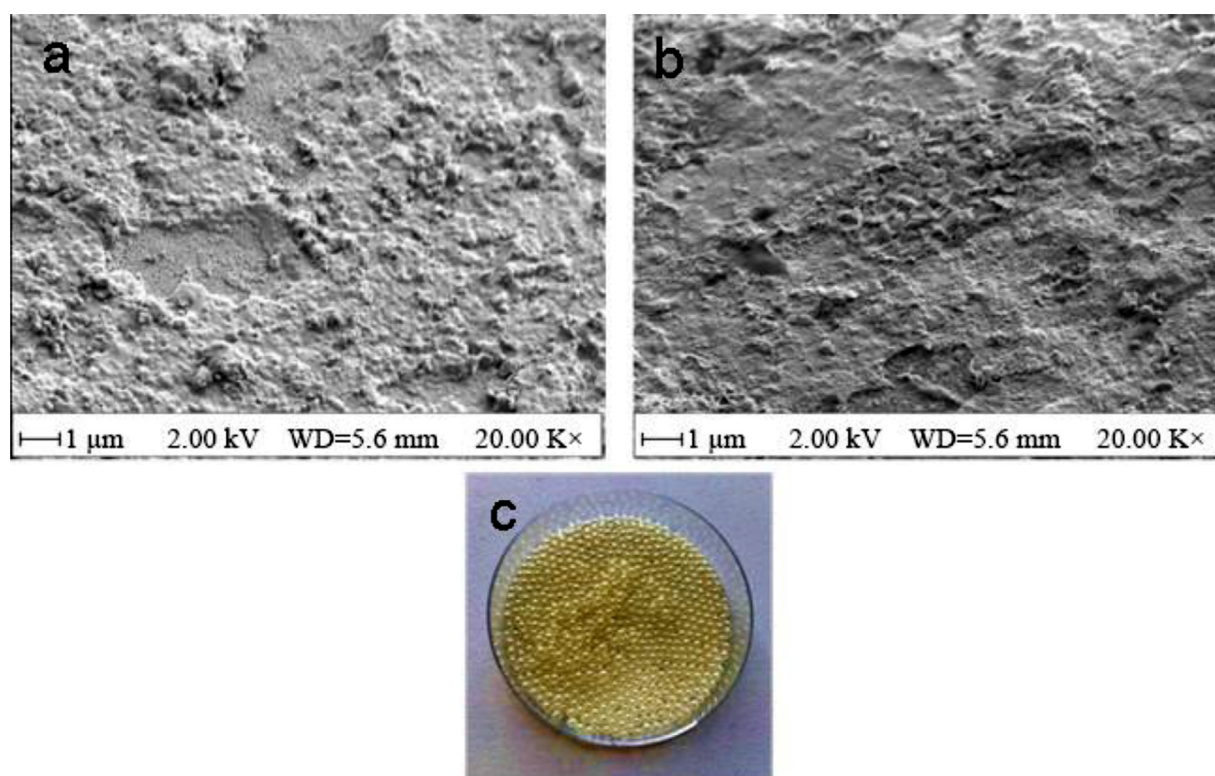
Fig. 4 – Scanning electron microscopy image of bismuth oxide glass bead that had no exposure to Microcystis aeruginosa (a), compared to one that had been exposed to a culture of Microcystis aeruginosa for 56 days showing no degradation or biofilm formation (b), photograph of bismuth oxide-coated glass beads showing visual appearance (c) WD: Working distance.
