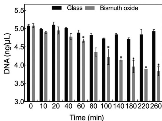
Fig. 5 – Quantification of free-floating Lambda genomic DNA after treatment with either bismuth oxide-coated glass beads or glass beads. Values are mean ( n=3 ) and error bars represent \pm 1 standard deviation. Time points where the amount of DNA is significantly lower ( p < 0.05 ) are represented by *.
