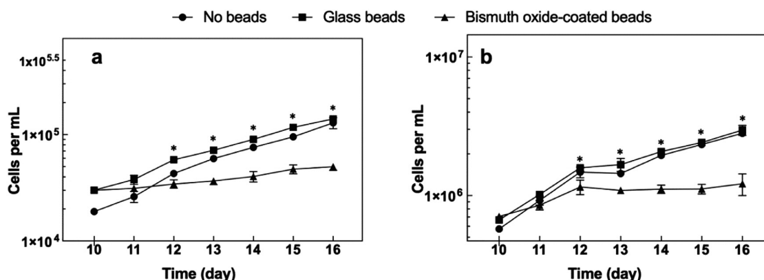
Fig. 2 – Cell density of the cyanobacteria Microcystis aeruginosa (a) and Anabaena sp. (b) following addition at day 10 of either bismuth oxide-coated glass beads, glass beads or no beads. Cyanobacteria were actively growing at the time of treatment. Values represent means ( n=3 ) and error bars represent \pm 1 standard deviation. Days at which the number of cells exposed to bismuth oxide are statistically significantly lower ( p < 0.001 ) than controls are indicated by *.
