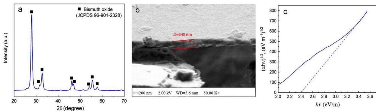
Fig. 1 – Selected results of analysis of bismuth oxide-coated glass beads: XRD pattern (a), cross-sectional SEM (b), Tauc plot method band gap calculation (c). WD = Working distance.
