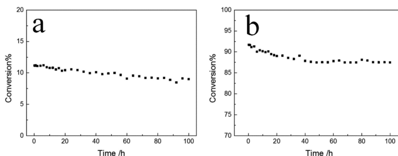
Fig. S2 – Catalyst life of Cu 0.7 Mn 2 Ce 0.3 O x /sepiolite: catalytic temperature was 190°C(a) and 270°C(b). Should be revised to
