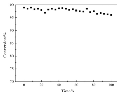
Fig. S2 – Catalyst life of Cu 0.7 Mn 2 Ce 0.3 O x /HTS-1
